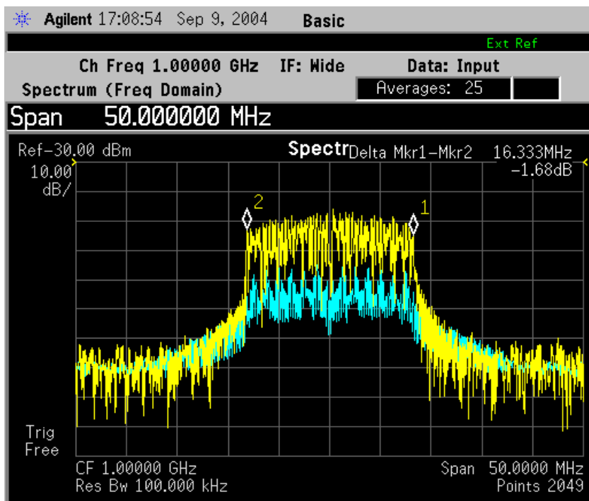
Figure 2-76 Spectrum Measurement - Spectrum Zoom View with Opt. 122-80 MHz Bandwidth Digitizer Hardware
