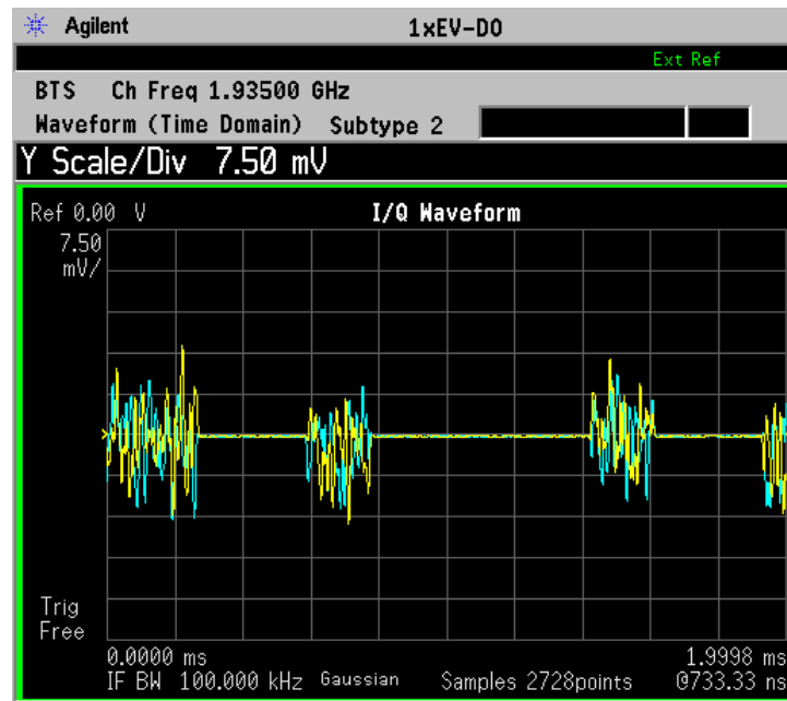
Figure 3-41 Waveform Measurement - I and Q Waveform View
