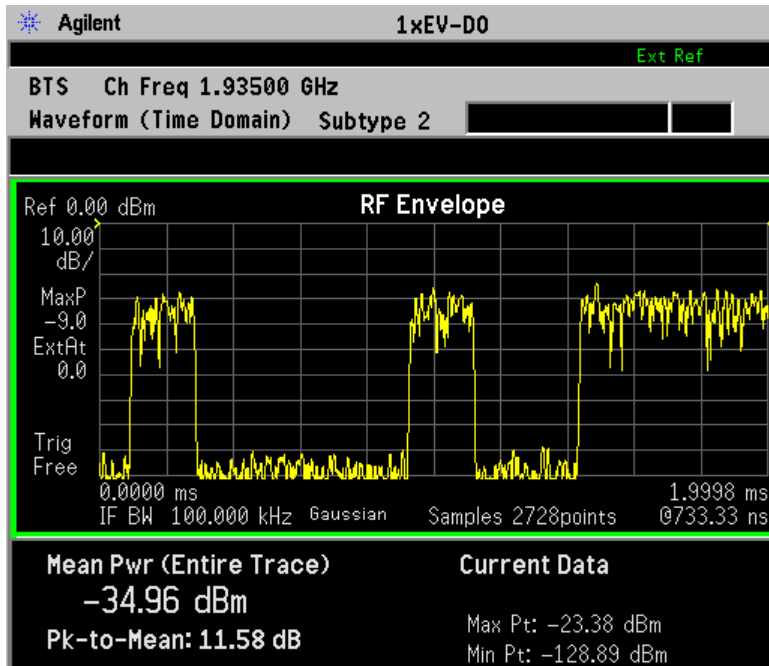
Figure 2-93 Waveform Measurement - RF Envelope (Default View)
