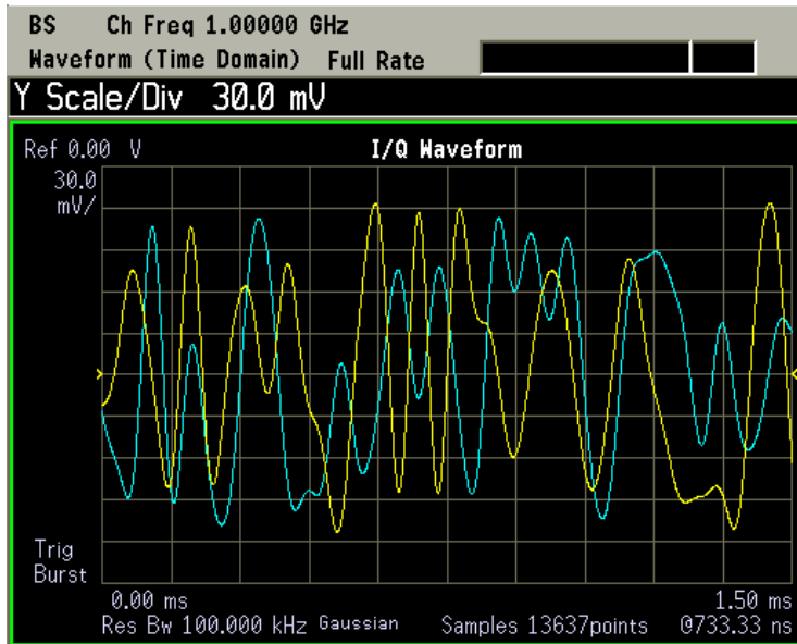
Figure 2-100 Waveform Measurement - I/Q Waveform View
