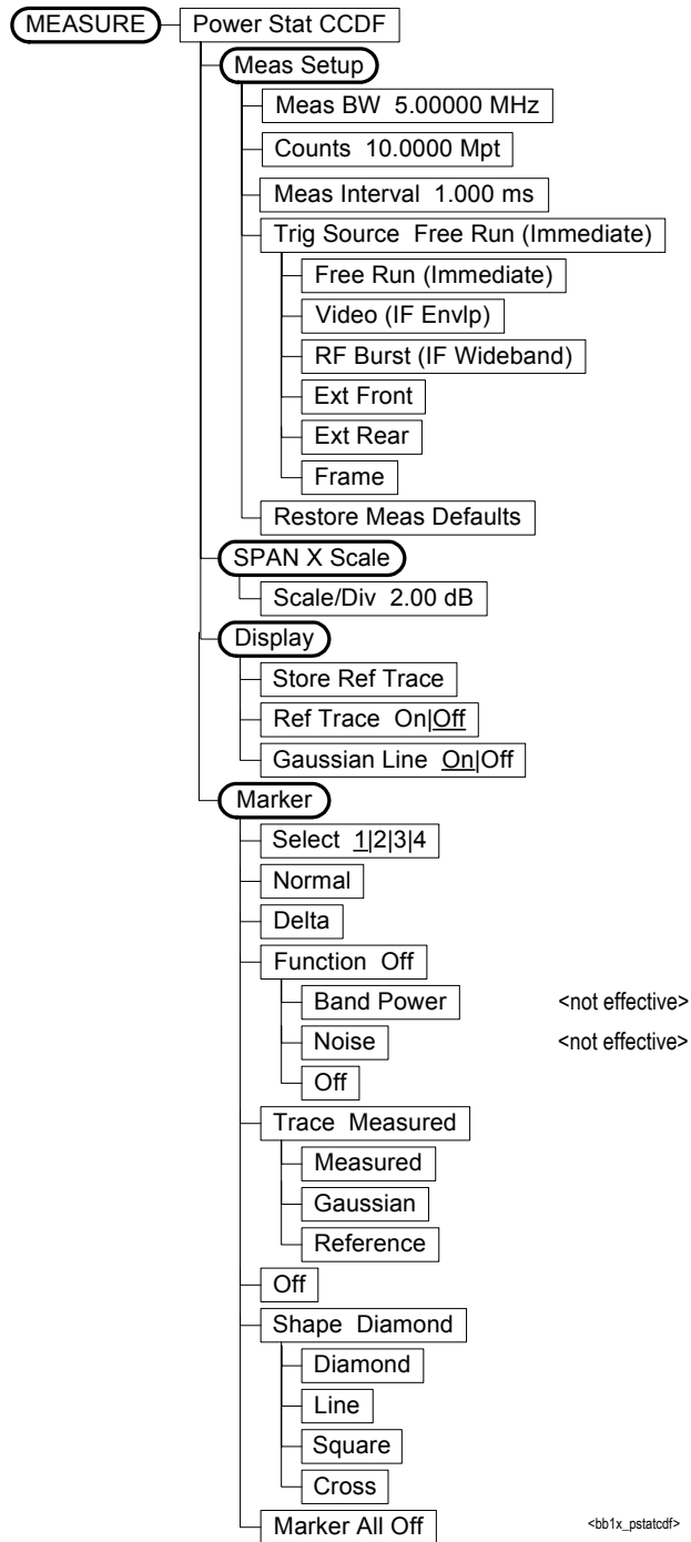
Figure 6-17 Power Statistics CCDF Measurement Key Flow
