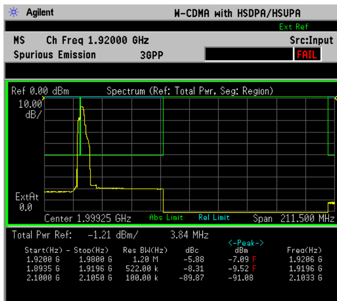
Figure 2-70 Spectrum Measurement - I and Q Waveform View (for E4406A)
