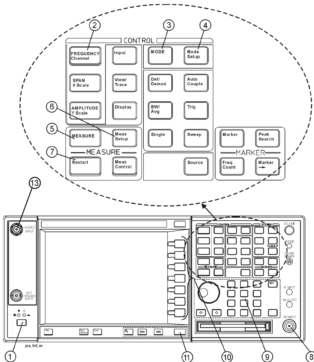
Figure 2-2 Selected PSA Series Front Panel Feature Locations
