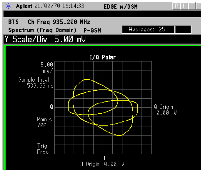
Figure 2-75 Spectrum Measurement - I/Q Polar View (for E4406A)
