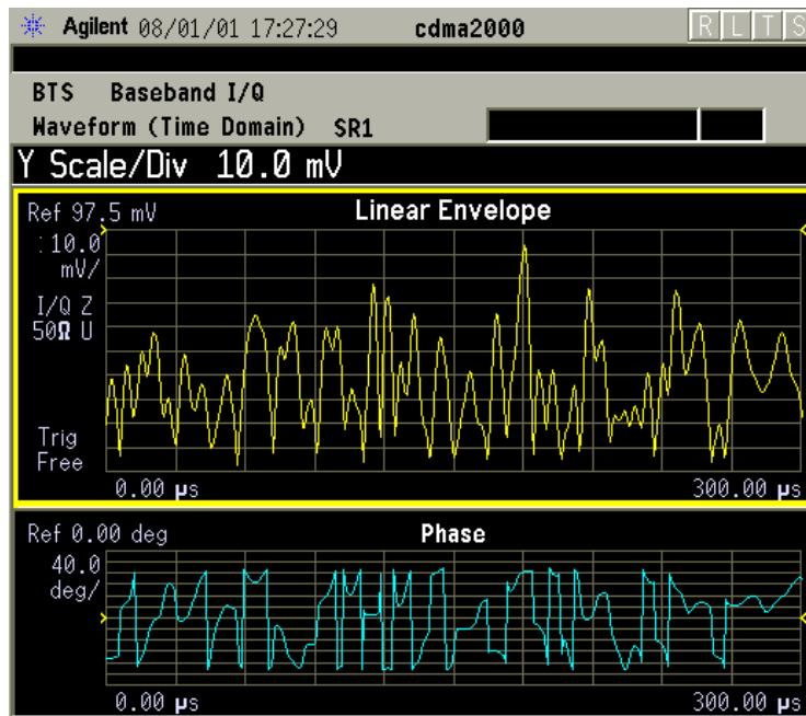
Figure 2-95 Waveform Measurement - Linear Envelope View
