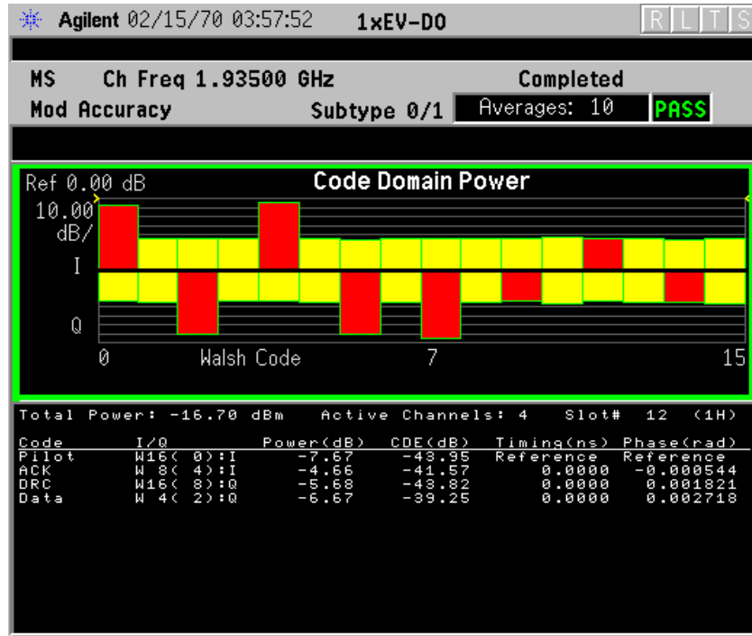
Figure 3-21 Reverse Link Modulation Accuracy - Code Domain Power View
