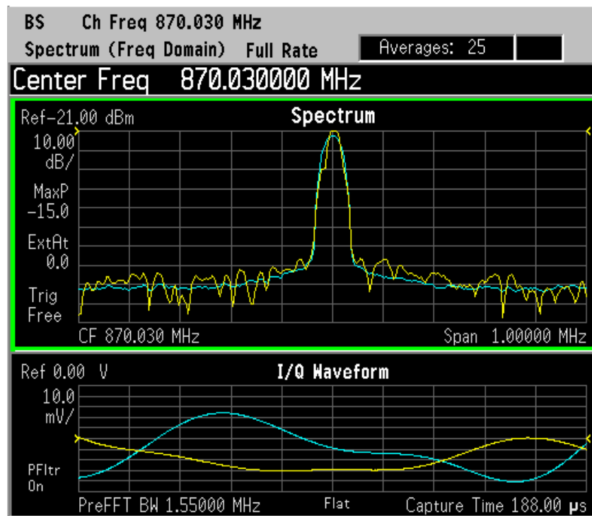
Figure 2-56 Spectrum Measurement - Spectrum and I/Q Waveform (Default View)
