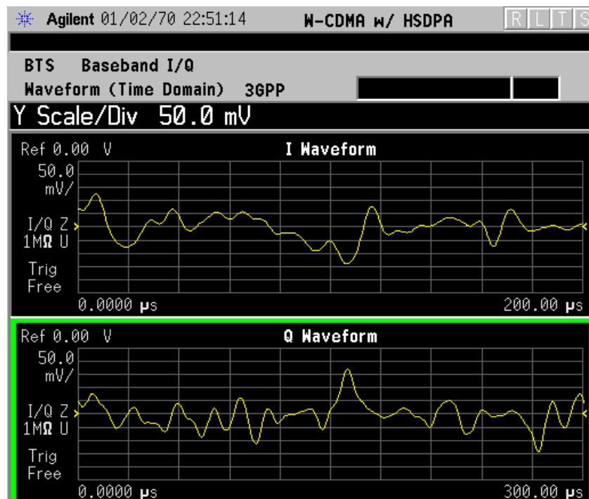
Figure 2-109 Waveform Measurement - I and Q Waveform View
