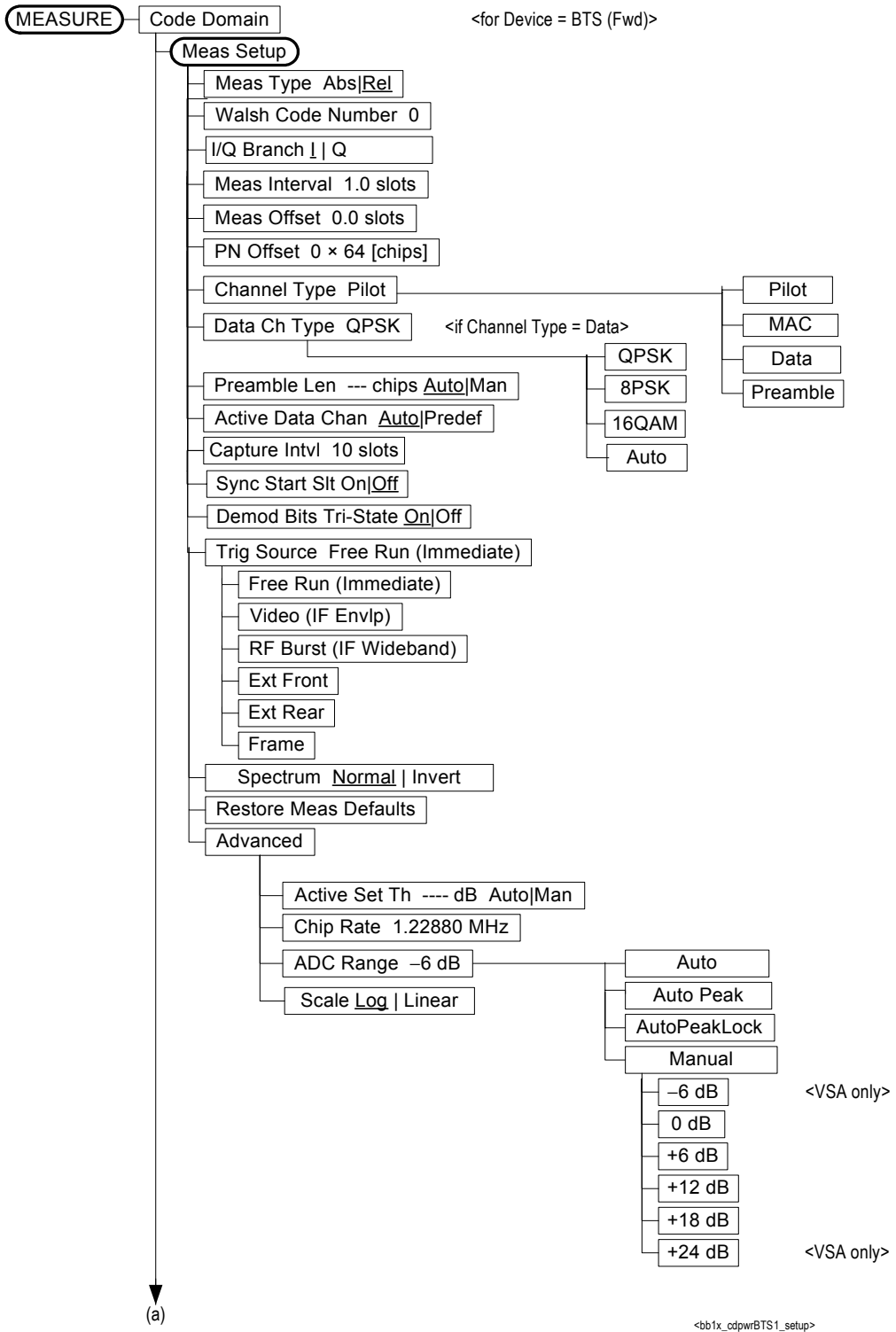
Figure 6-6 Forward Link Code Domain Measurement Key Flow (1 of 4)
