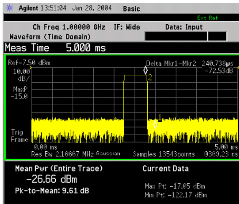
Figure 2-116 Waveform Measurement - RF Envelope View with Opt. 122–80 MHz Bandwidth Digitizer Hardware
