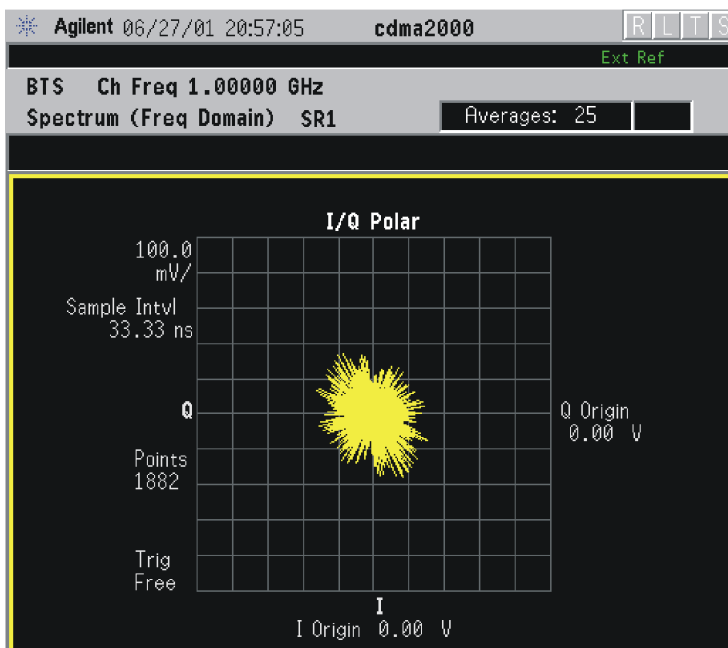
Figure 2-73 Spectrum Measurement - I/Q Polar View (for E4406A)
