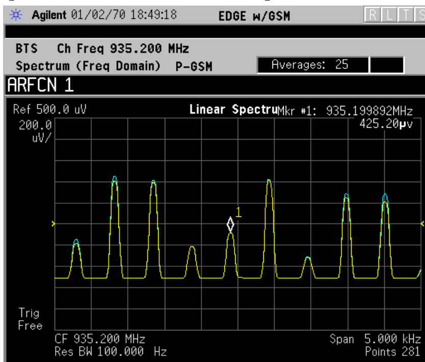
Figure 2-63 Spectrum Measurement - Linear Spectrum View (for E4406A)
