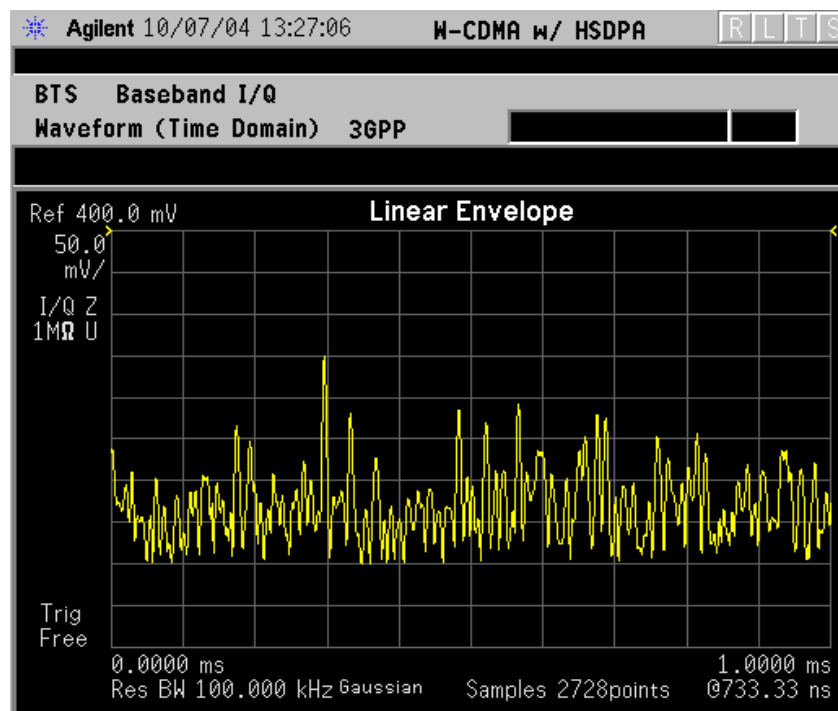
Figure 2-96 Waveform Measurement - Linear Envelope View
