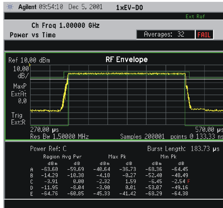
Figure 3-23 Power vs. Time Measurement - Rise & Fall View
