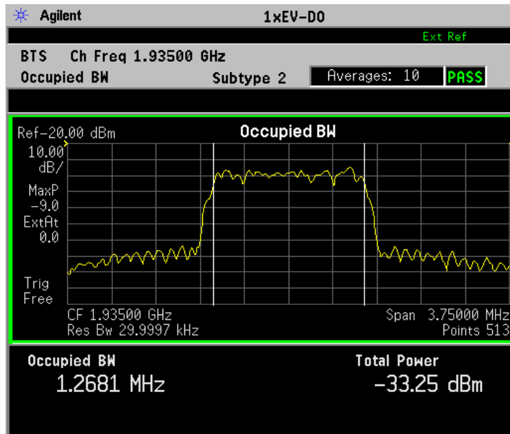
Figure 2-40 Occupied Bandwidth Measurement Result
