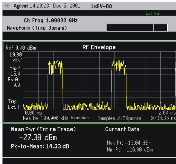
Figure 3-38 Waveform Measurement - RF Envelope (Default View)
