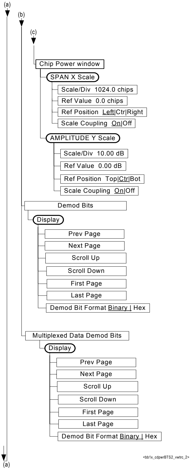
Figure 6-8 Forward Link Cod Domain Measurement Key Flow (3 of 4)
