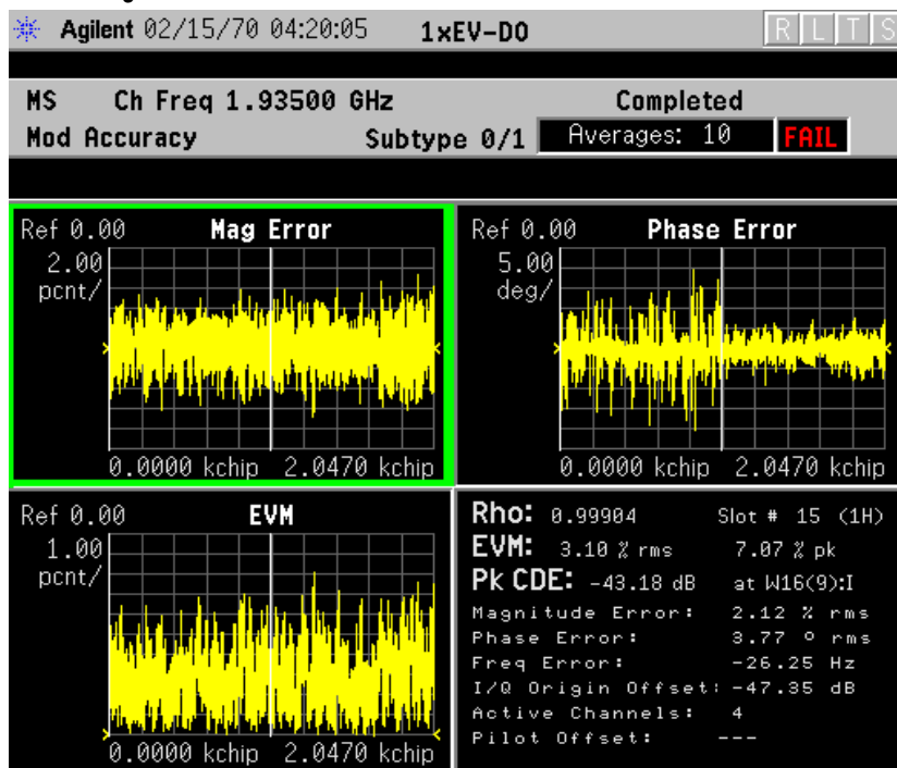
Figure 2-37 Reverse Link Modulation Accuracy Measurement Result - I/Q Error Quad View
