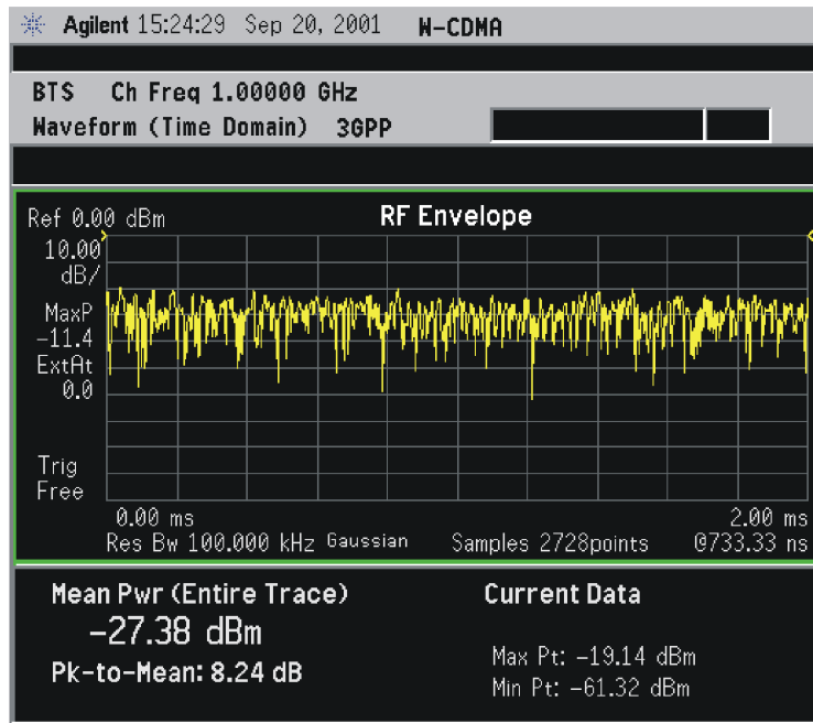
Figure 2-92 Waveform Measurement - RF Envelope (Default View)
