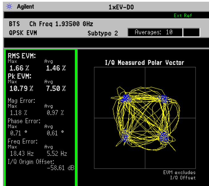
Figure 3-24 QPSK EVM Measurement - I/Q Polar Vector View
