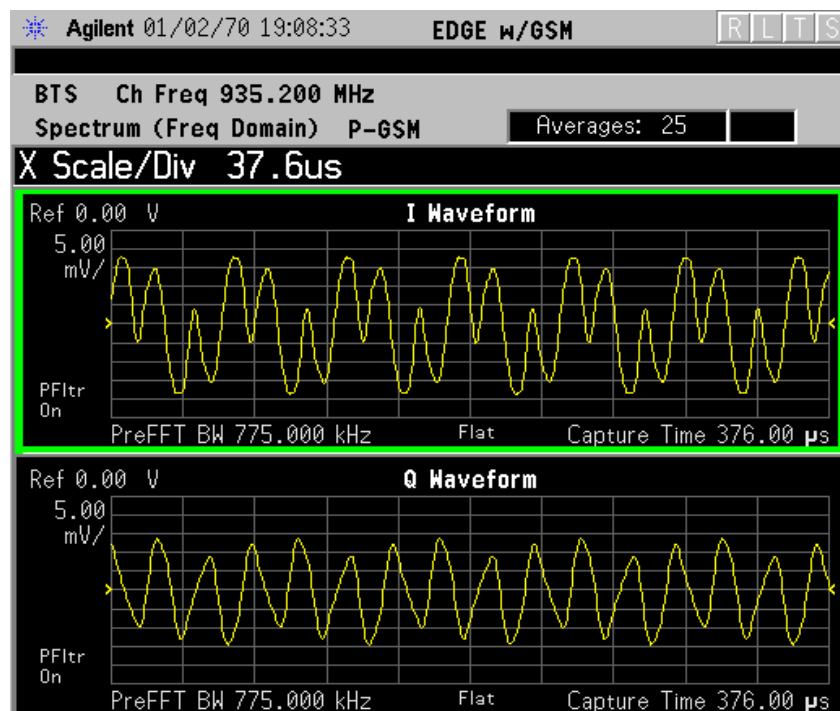
Figure 3-31 Spectrum Measurement - I and Q Waveform View (for E4406A)
