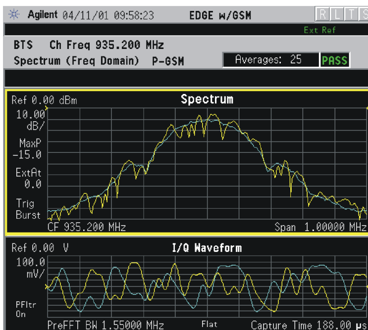
Figure 2-54 Spectrum Measurement - Spectrum and I/Q Waveform (Default View)
