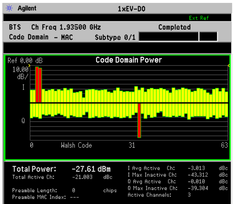
Figure 2-7 Forward Link Code Domain Result - MAC Channels Subtype 0/1
