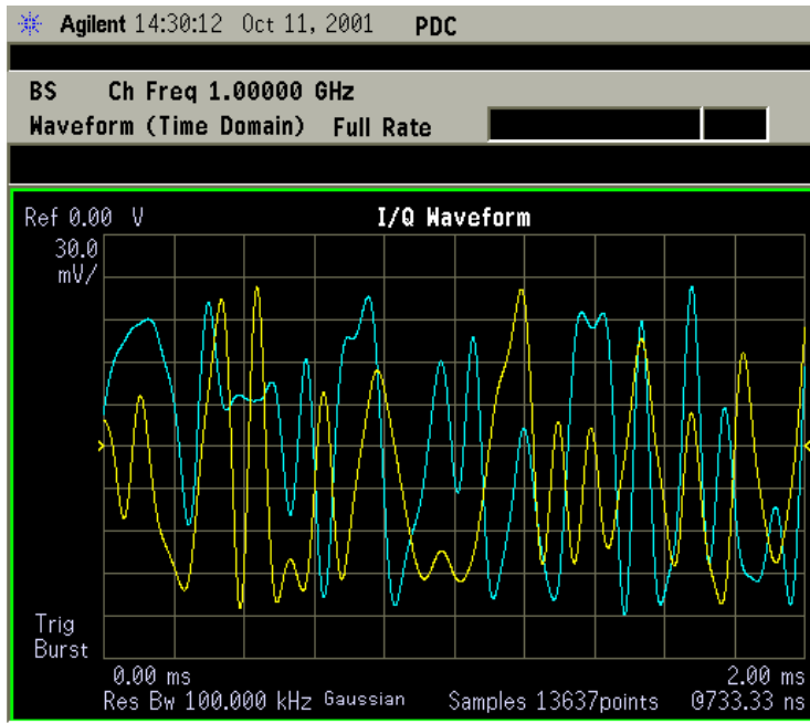
Figure 2-101 Waveform Measurement - I/Q Waveform View
