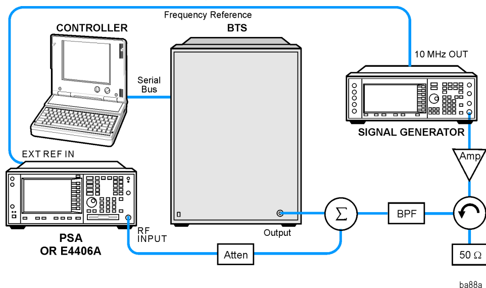
Figure 2-85 Waveform Measurement System
