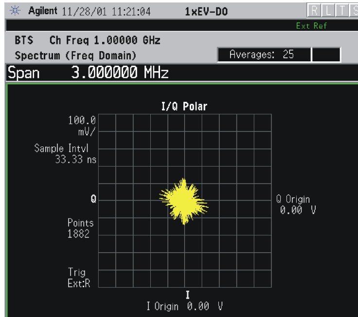
Figure 3-32 Spectrum Measurement - I/Q Polar View (for E4406A)
