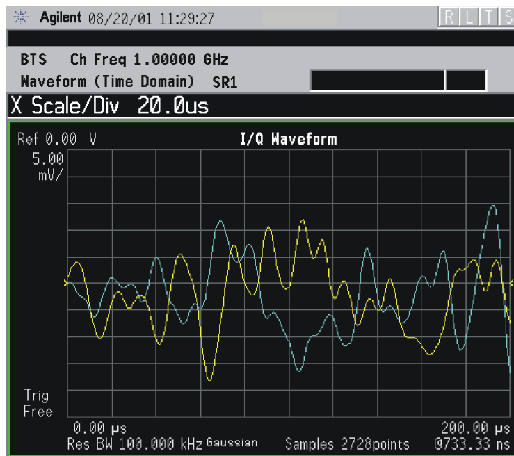
Figure 2-103 Waveform Measurement - I/Q Waveform View
