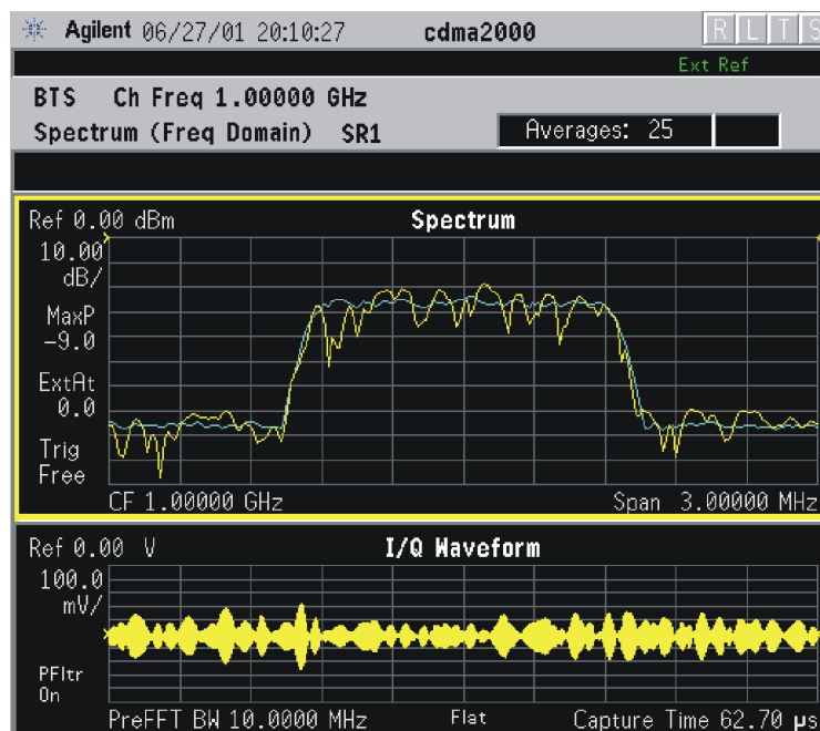
Figure 2-56 Spectrum Measurement - Spectrum and I/Q Waveform (Default View)
