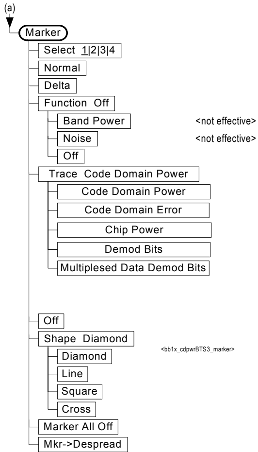
Figure 6-9 Forward Link Code Domain Measurement Key Flow (4 of 4)
