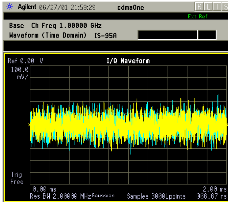
Figure 2-102 Waveform Measurement - I/Q Waveform View
