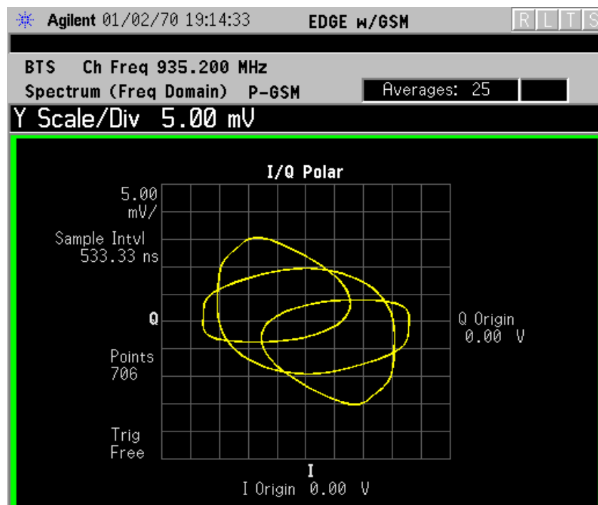
Figure 3-33 Spectrum Measurement - I/Q Polar View (for E4406A)
