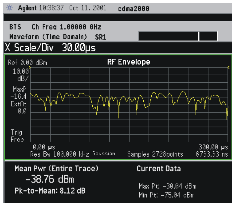
Figure 2-91 Waveform Measurement - RF Envelope (Default View)
