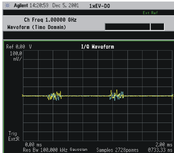
Figure 3-40 Waveform Measurement - I/Q Waveform View
