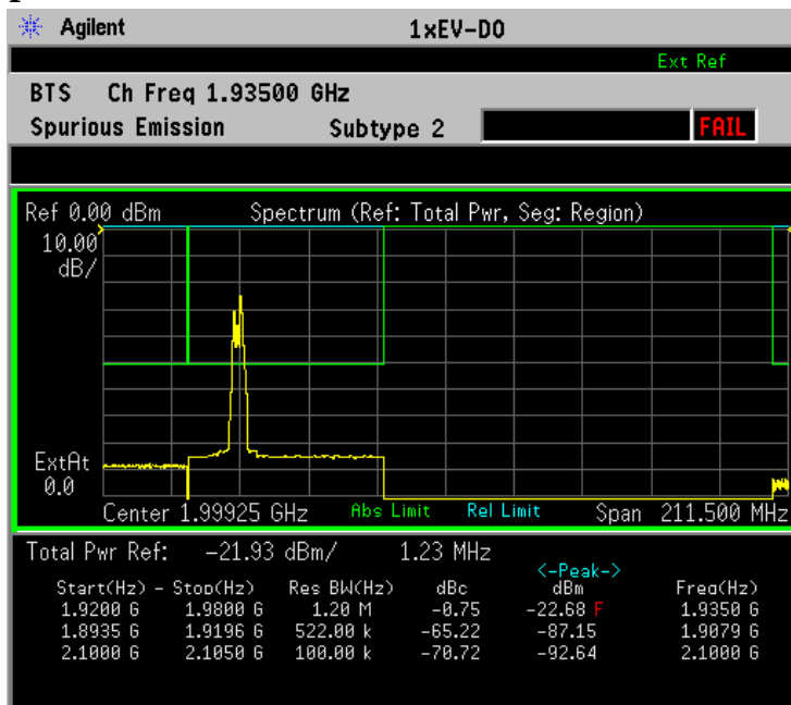
Figure 2-82 Spectrum Emission Mask Measurement Result - Region View
