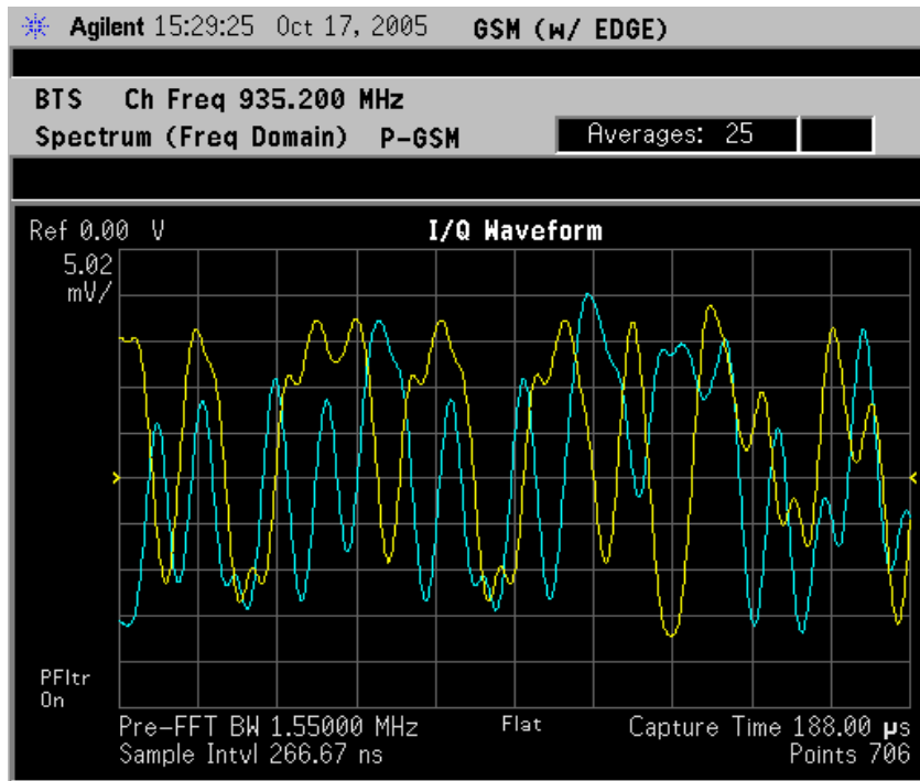
Figure 2-60 Spectrum (Time Domain) Measurement - I/Q Waveform Result
