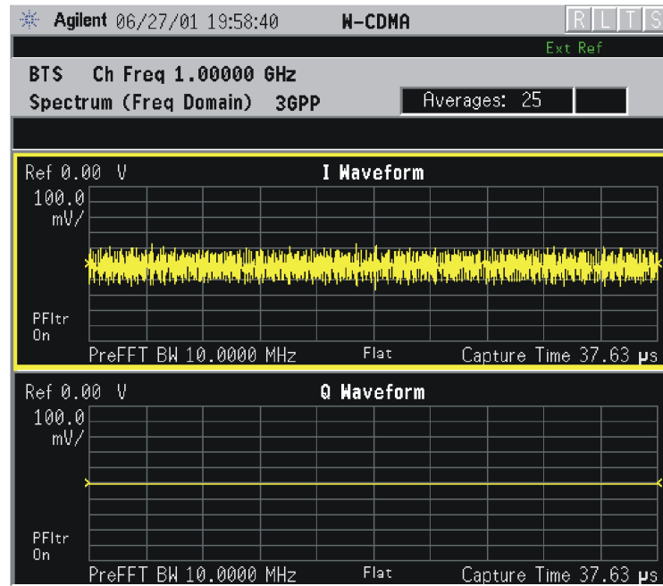
Figure 2-67 Spectrum Measurement - I and Q Waveform View (for E4406A)
