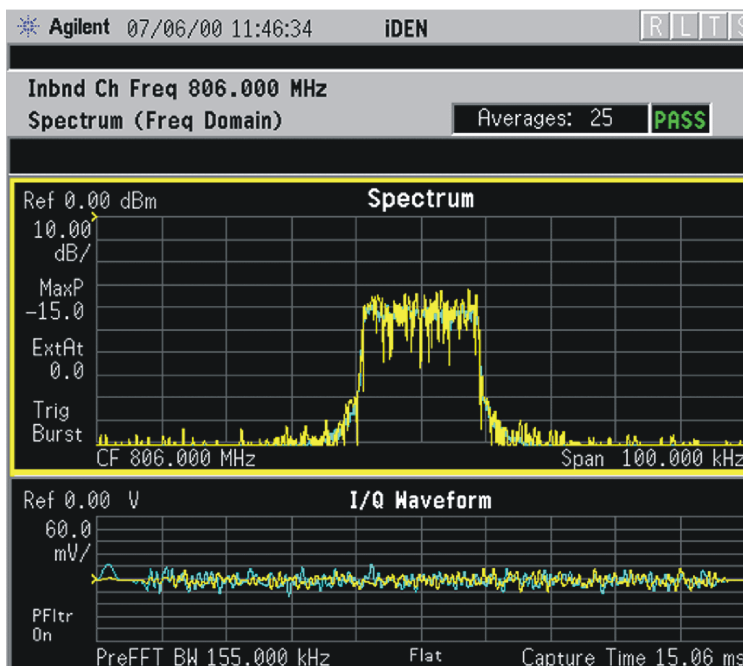
Figure 2-55 Spectrum Measurement - Spectrum and I/Q Waveform (Default View)
