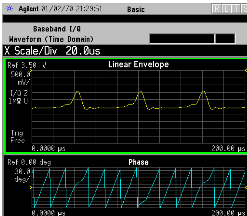
Figure 2-94 Waveform Measurement - Linear Envelope View
