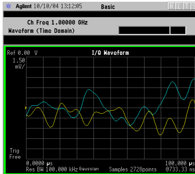
Figure 3-39 Waveform Measurement - I/Q Waveform View
