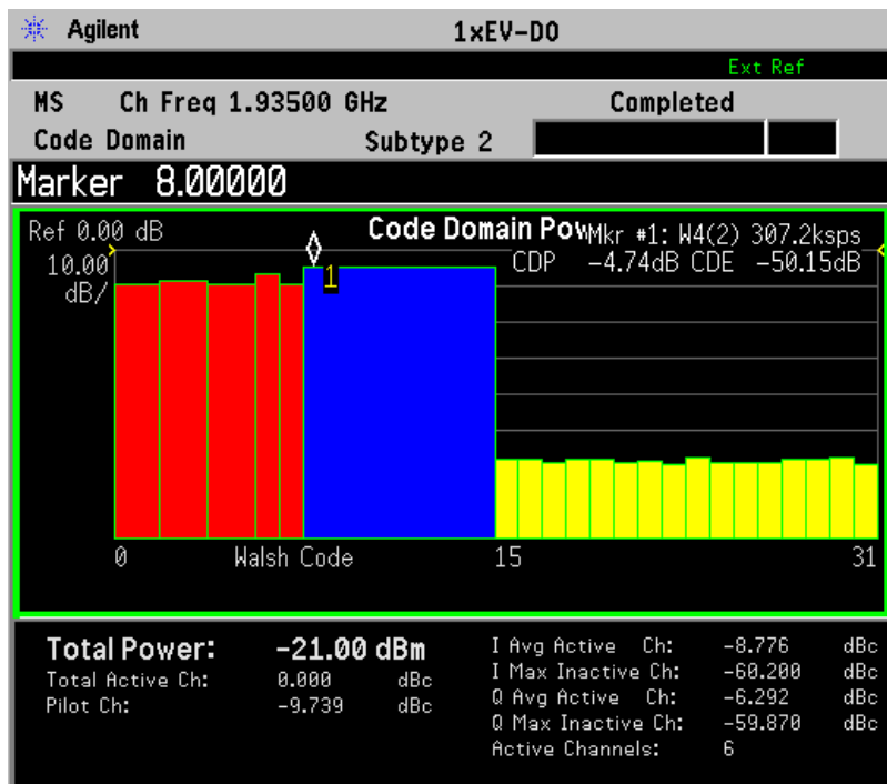
Figure 2-18 Reverse Link Code Domain Result - I/Q Combined with Marker)
