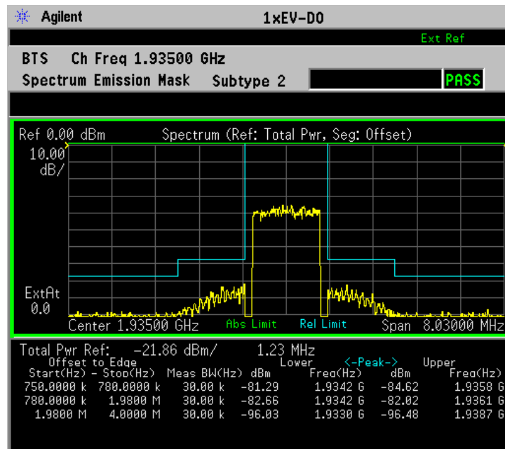
Figure 3-34 Spurious Emissions Measurement - Offset View
