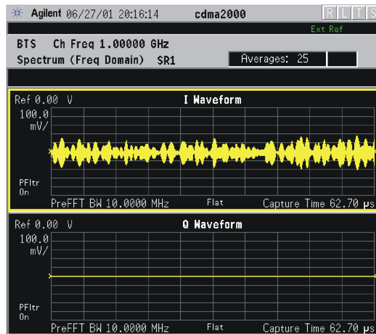
Figure 2-68 Spectrum Measurement - I and Q Waveform View (for E4406A)
