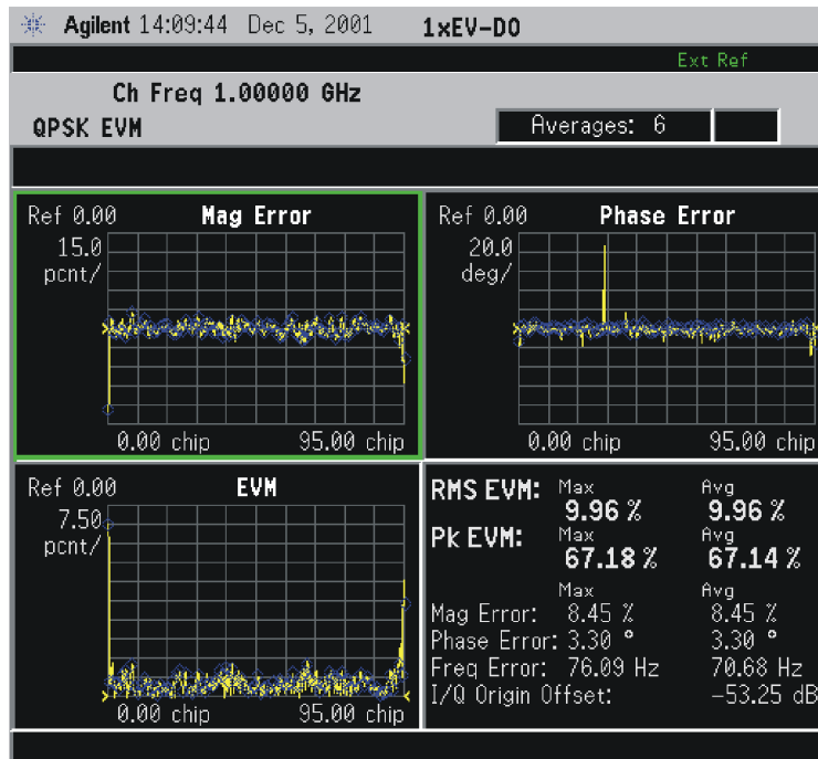
Figure 3-26 QPSK EVM Measurement - I/Q Error Quad View
