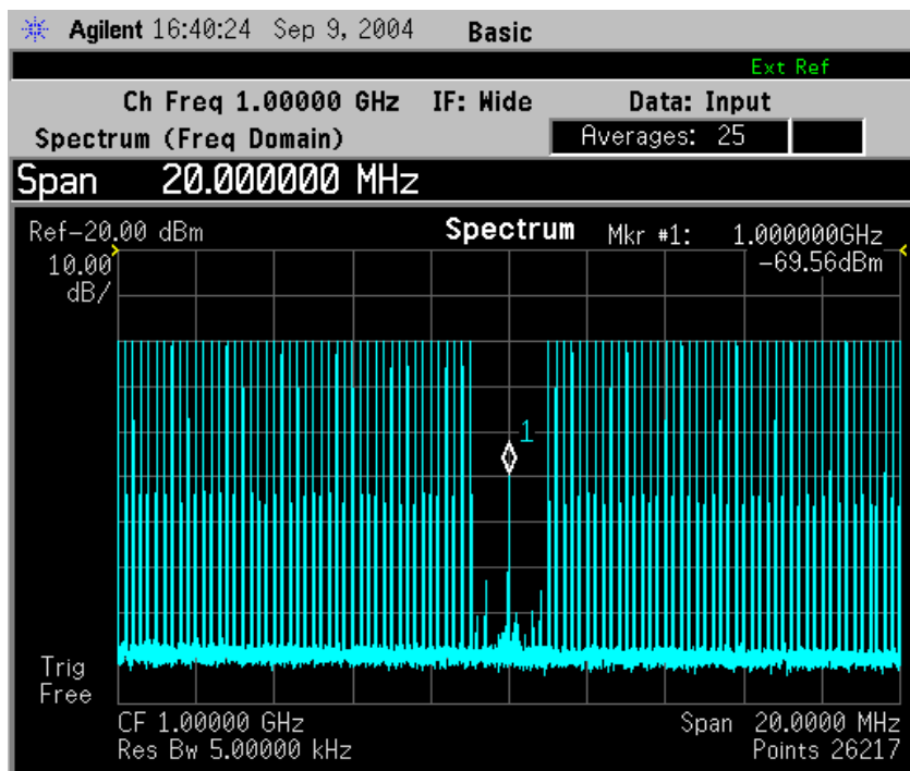
Figure 2-78 Spectrum Measurement - Spectrum View with Opt. 122– 80 MHz Bandwidth Digitizer Hardware
