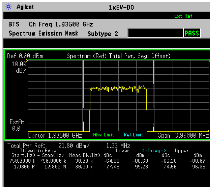
Figure 2-83 Spectrum Emission Mask Measurement Result - ACP View
