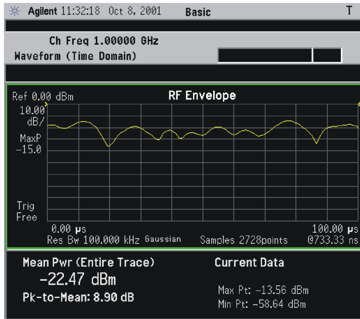
Figure 2-88 Waveform Measurement - RF Envelope (Default View)
