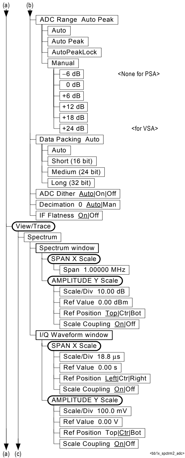
Figure 6-30 Spectrum (Freq Domain) Measurement Key Flow (2 of 4)
