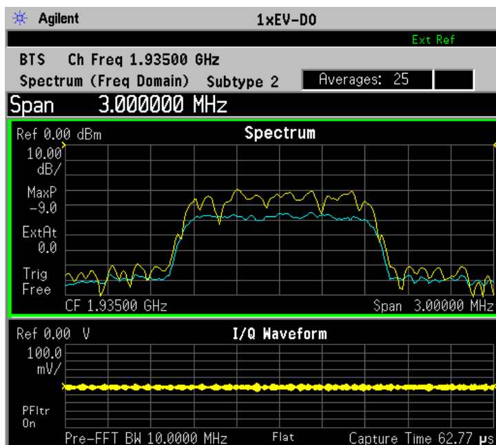
Figure 2-58 Spectrum Measurement - Spectrum and I/Q Waveform (Default View)
