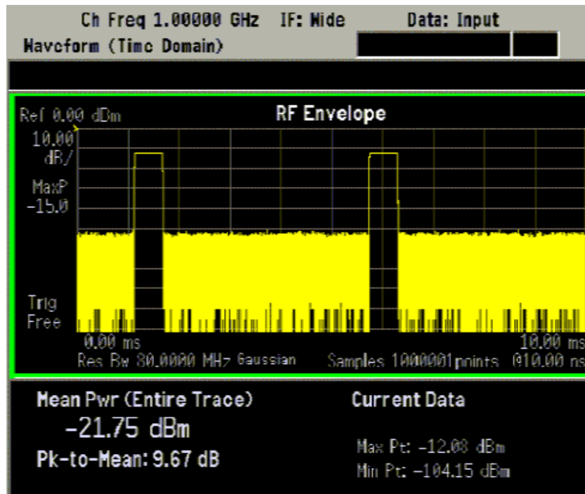
Figure 2-115 Waveform Measurement - RF Envelope View with Opt. 122– 80 MHz Bandwidth Digitizer Hardware
