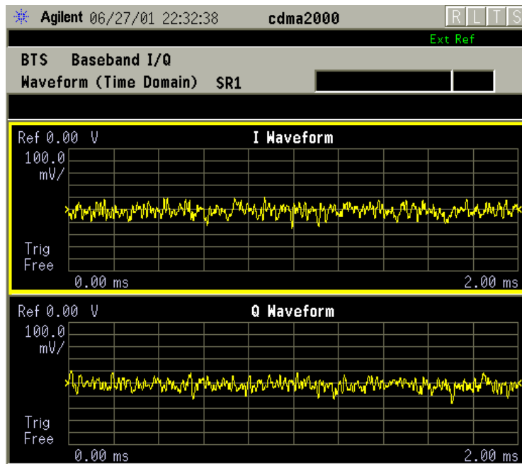
Figure 2-108 Waveform Measurement - I and Q Waveform View
