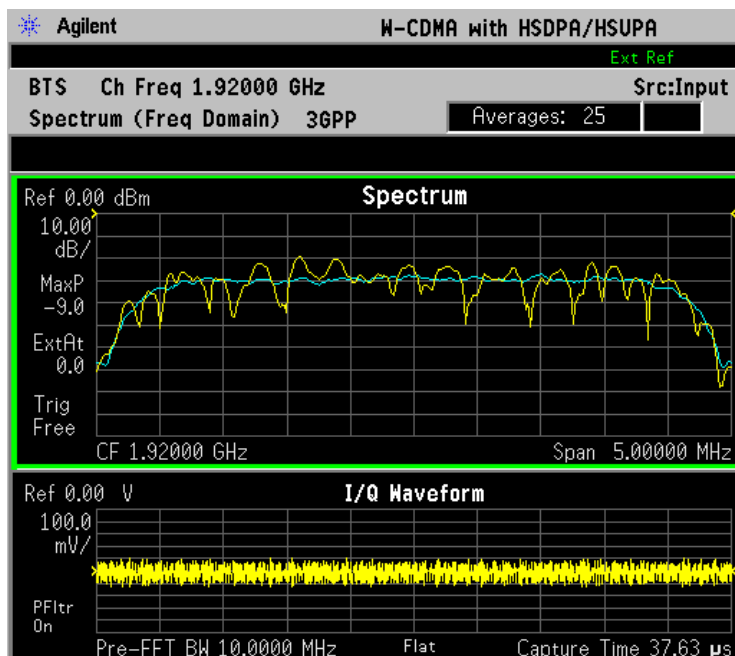
Figure 2-57 Spectrum Measurement - Spectrum and I/Q Waveform (Default View)
