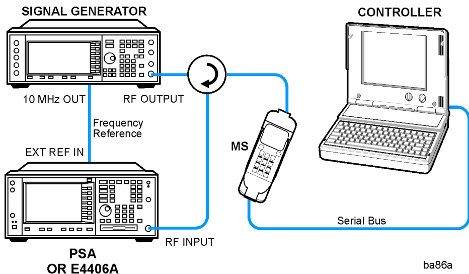
Figure 2-84 Waveform Measurement System
