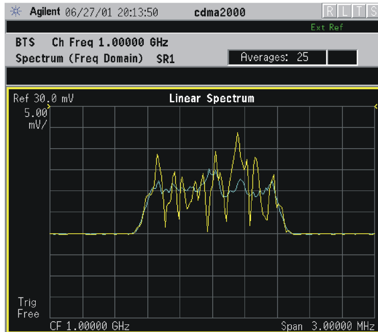
Figure 2-64 Spectrum Measurement - Linear Spectrum View (for E4406A)
