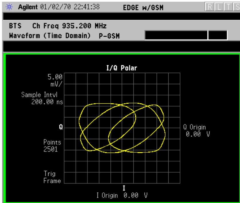
Figure 2-111 Waveform Measurement - I/Q Polar View
