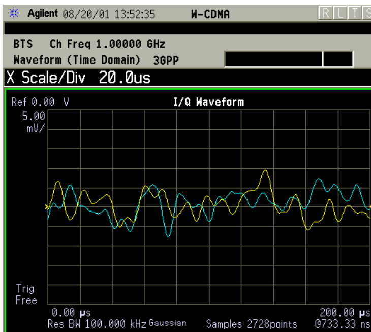
Figure 2-104 Waveform Measurement - I/Q Waveform View
