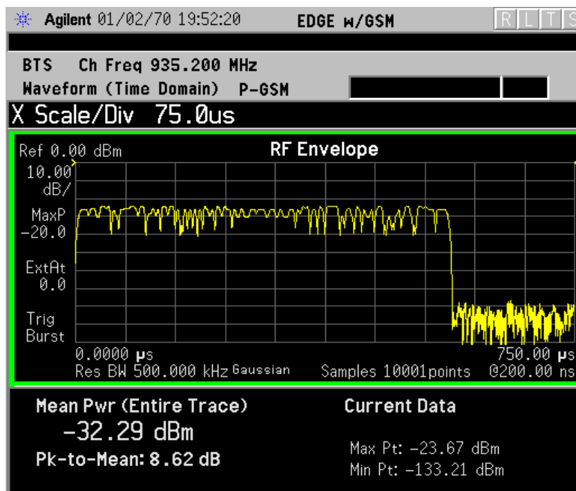
Figure 2-87 Waveform Measurement - RF Envelope (Default View)
