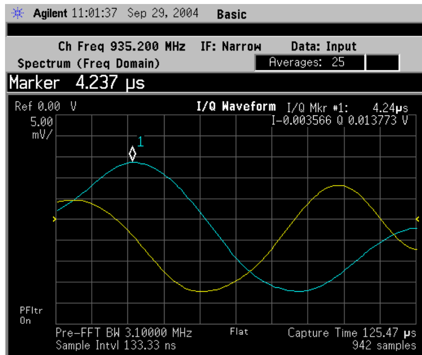
Figure 2-59 Spectrum (Time Domain) Measurement - I/Q Waveform Result
