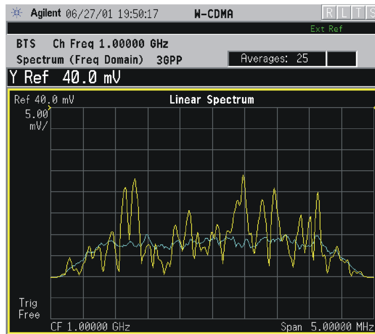
Figure 2-62 Spectrum Measurement - Linear Spectrum View (for E4406A)
