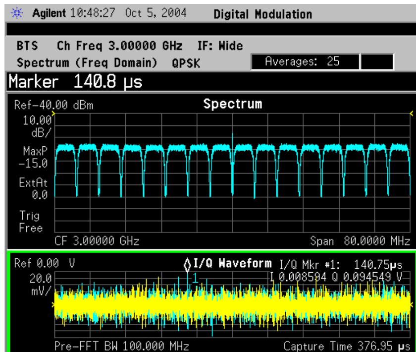
Figure 2-79 Spectrum Measurement - Spectrum Zoom View with Opt. 122–80 MHz Bandwidth Digitizer Hardware
