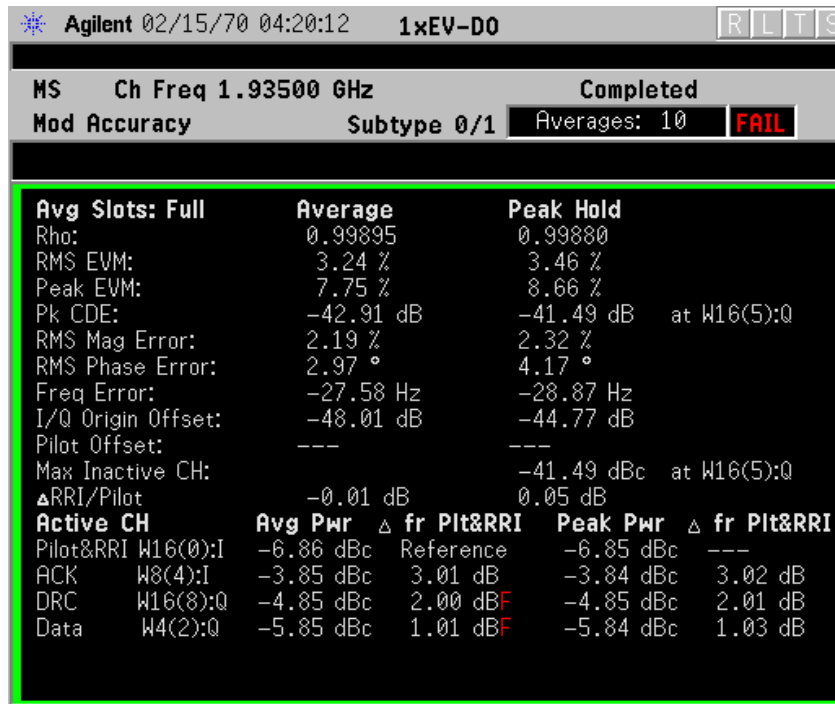
Figure 2-36 Reverse Link Modulation Accuracy Measurement Result - Peak/Average Metrics View
