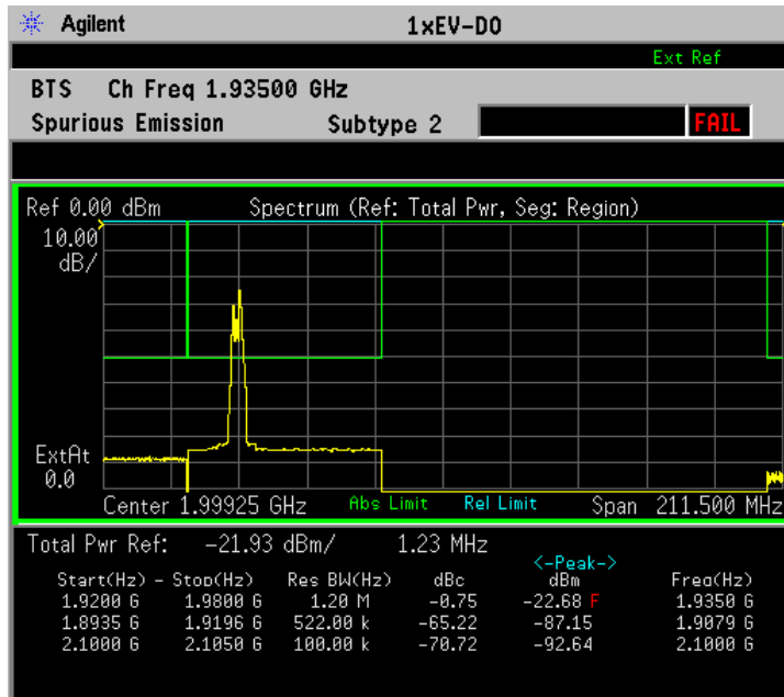
Figure 3-35 Spurious Emissions and ACP Measurement - All Regions View
