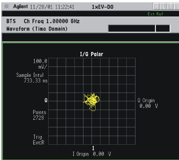
Figure 2-114 Waveform Measurement - I/Q Polar View
