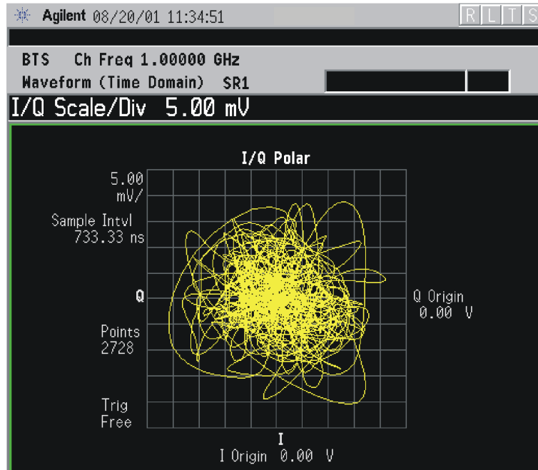
Figure 2-112 Waveform Measurement - I/Q Polar View
