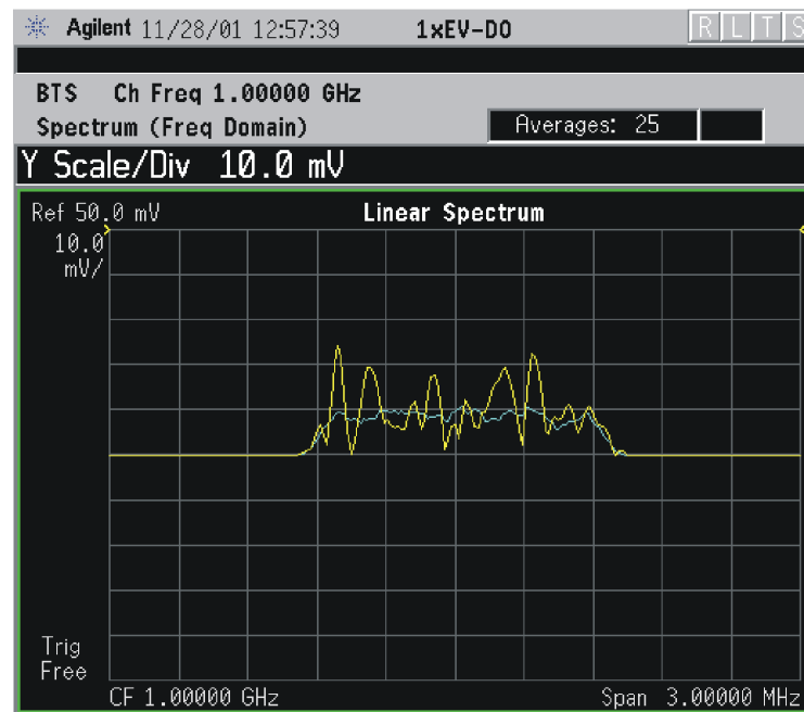
Figure 2-65 Spectrum Measurement - Linear Spectrum View (for E4406A)
