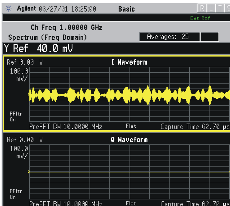
Figure 2-66 Spectrum Measurement - I and Q Waveform View (for E4406A)
