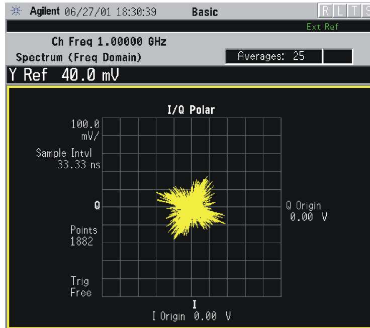
Figure 2-71 Spectrum Measurement - I/Q Polar View (for E4406A)
