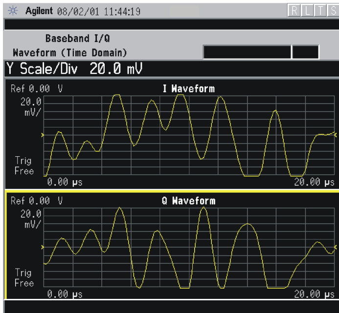
Figure 2-107 Waveform Measurement - I and Q Waveform View
