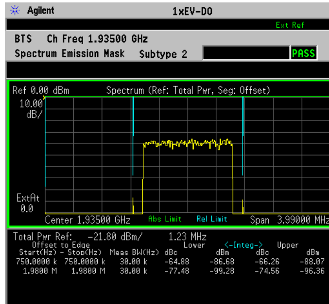
Figure 3-36 Spurious Emissions and ACP Measurement - ACP Mode View
