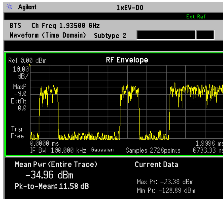
Figure 3-37 Waveform Measurement - RF Envelope (Default View)
