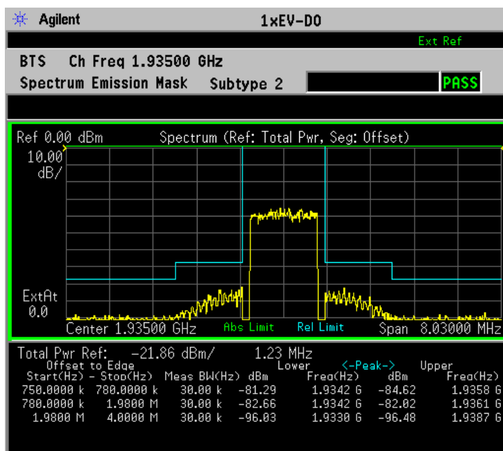
Figure 2-81 Spectrum Emission Mask Measurement Result - Offset (Default) View
