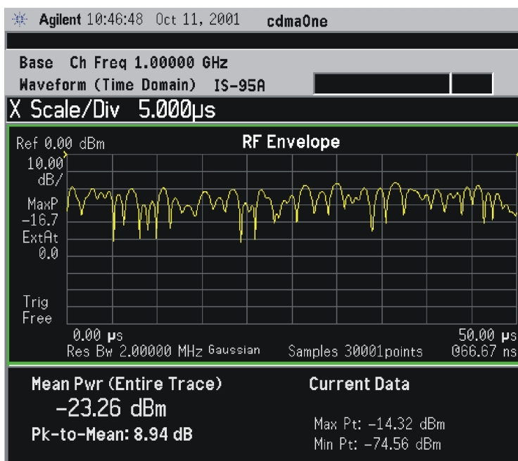
Figure 2-86 Waveform Measurement - RF Envelope (Default View)
